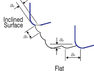
Finishing Parameter (Flat / Inclined Surface)
