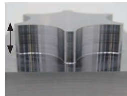
Tool after milling
