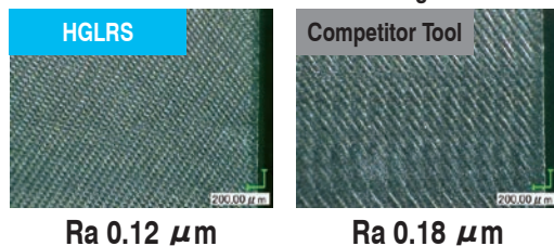
Surface condition after milling
