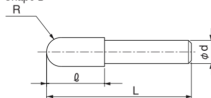
Shape B
