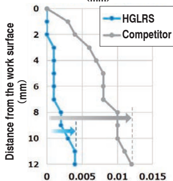
Deflection of the wall after milling ( \text{mm} )
