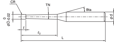
Shape A
