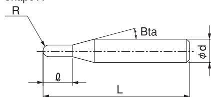
Shape A
