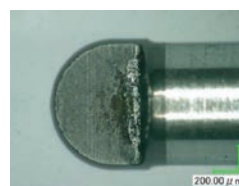
Tool after 45h of milling
